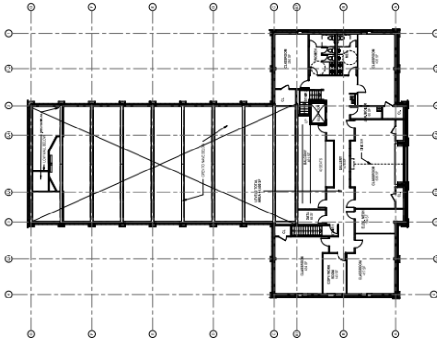
LEVEL 2 - FLOOR PLAN SCALE: 1/200
