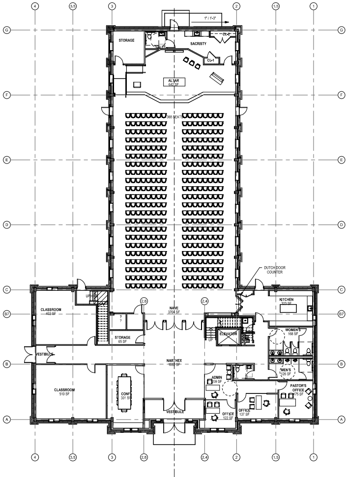
1 LEVEL 1 - FLOOR PLAN PRES-1 SCALE: 3/32" = 1'-0"
